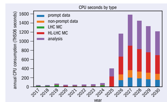
Fig. 2. CMS estimated disk space (left) and CPU resources (right) required for the high-luminosity LHC era, using the current computing model with parameters projected for the next 12 years. The vertical label “THS06” stands for Terra HEP SPEC 06, a standard measure of the performance of a CPU code used in high-energy physics.
