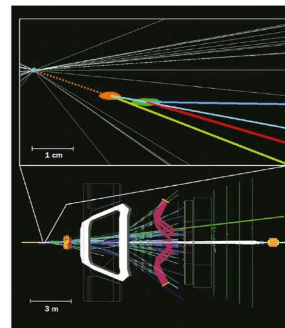
Side view of an event in the LHCb detector and an enlarged area close to the interaction point, showing the decay of a B meson produced in the proton–proton interaction.
