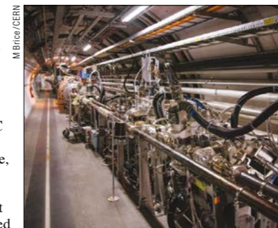
Left: one side of the TOTEM apparatus in the LHC tunnel. Right: dependence of \rho on energy, showing pp (blue) and p\bar{p} (green) data taken from the Particle Data Group and TOTEM measurements at 13 TeV (red). Contrary to the traditional QCD picture, based on results from the COMPETE collaboration, the rate of growth of \rho slows at high energies.
