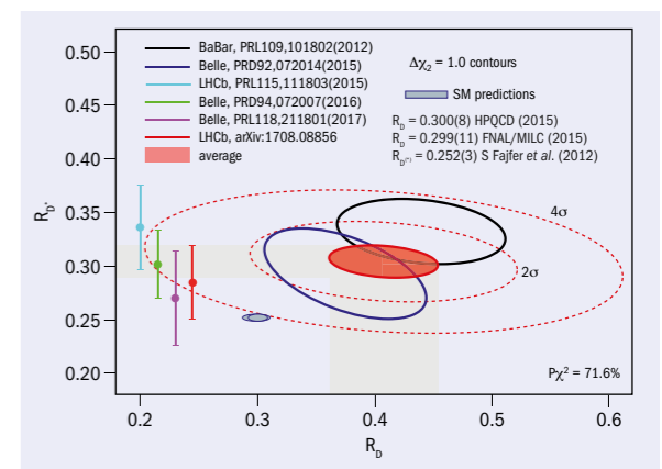
Fig. 2. Status of R_{D^*} and R_D measurements. The red ellipse represents the world average, including both the results from simultaneous measurements of R_D and R_{D^*} (black and blue ellipses) and separate measurements of R_{D^*} (points with error bars).
