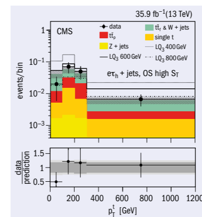
The distribution of the transverse momentum of the leading top-quark candidate in one of the search categories optimised for the LQ search by CMS (left), and the exclusion limits as a function of LQ mass and branching ratio into top+tau ( B=1 ) and bottom+neutrino ( B=0 ), reaching the TeV region (right).
