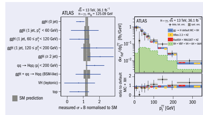
Left: the nine measured simplified template cross sections (blue markers) normalised to the Standard Model expectation (grey bands). Right: measured Higgs boson transverse momentum differential cross section (data points) compared to three predictions for gluon-gluon fusion (coloured bands), and the predicted sum of weak-boson fusion and associated production with vector bosons as well as bottom- and top-quark pairs.
