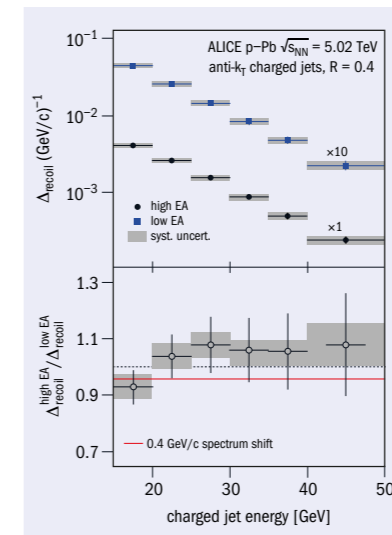
Background-subtracted recoil jet rates \Delta_{recoil} in p-Pb collisions with high and low event activity (EA), top, and the ratio of the two measurements (bottom). The ratio is compatible with unity, indicating no significant energy loss for jets in p-Pb collisions with large EA.
