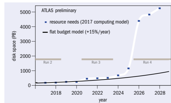
Fig. 1. The estimated disk-space requirements (left) and CPU resources (right) of the ATLAS experiment for period the 2018 to 2028 for both data and simulation processing. The blue points are estimates based on the current software performance estimates, while the solid line shows the amount of resources expected to be available if a flat-funding scenario is assumed, which implies an increase of 20% per year based on the current technology trends.
