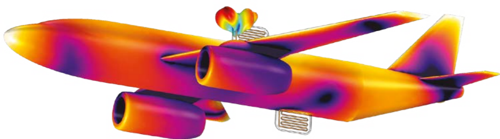
Visualization of the electric field norm and 3D far field due to a transmitting antenna. Antennas are intentionally large in this tutorial model.
