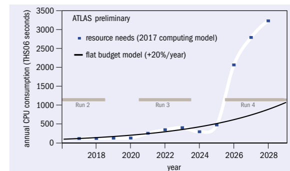
Fig. 1. The estimated disk-space requirements (left) and CPU resources (right) of the ATLAS experiment for period the 2018 to 2028 for both data and simulation processing. The blue points are estimates based on the current software performance estimates, while the solid line shows the amount of resources expected to be available if a flat-funding scenario is assumed, which implies an increase of 20% per year based on the current technology trends.
