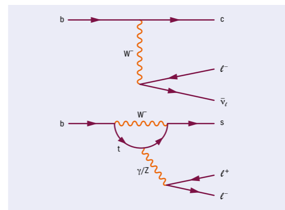
Fig. 1. Feynman diagrams in the Standard Model for two classes of processes relevant to the study of lepton universality in heavy quarks: a charged-current b \rightarrow c\ell^-\bar{\nu}_\ell tree-level transition (top) and a neutral-current b \rightarrow s\ell^+\ell^- loop-level transition (bottom).
