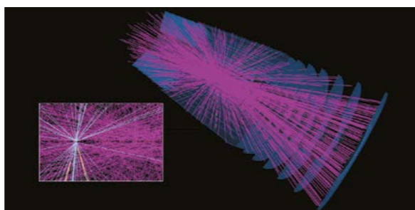
Fig. 3. The high-luminosity LHC upgrade will produce around 200 simultaneous proton–proton collisions in a single bunch crossing, illustrated by a simulated event for ATLAS.
