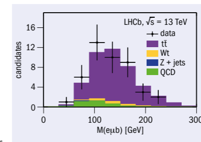
Selected events as a function of the invariant mass of the dilepton and b-jet system, with the signal component shown in purple.
