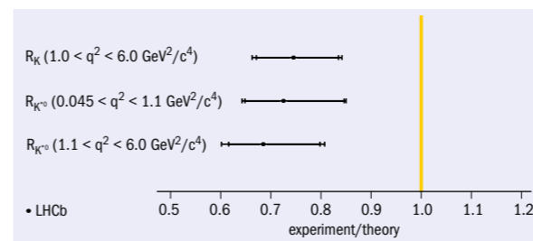
Fig. 3. LHCb measurements of the lepton universality ratios R_K and R_{K^*} . BaBar and Belle have made similar measurements, although with larger uncertainties.
