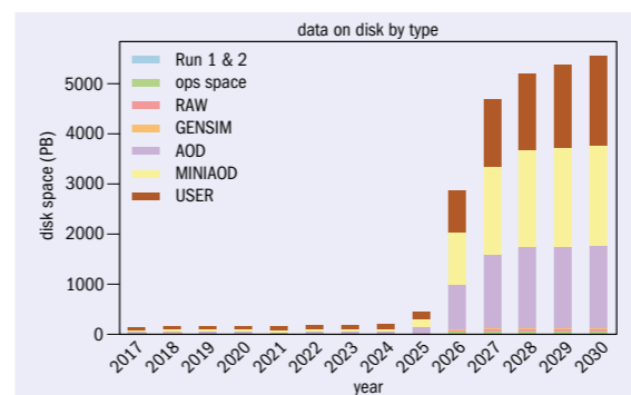
Fig. 2. CMS estimated disk space (left) and CPU resources (right) required for the high-luminosity LHC era, using the current computing model with parameters projected for the next 12 years. The vertical label “THS06” stands for Terra HEP SPEC 06, a standard measure of the performance of a CPU code used in high-energy physics.
